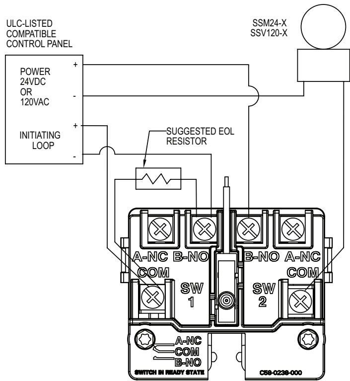
FIGURE 7. WFDNA WIRING:
