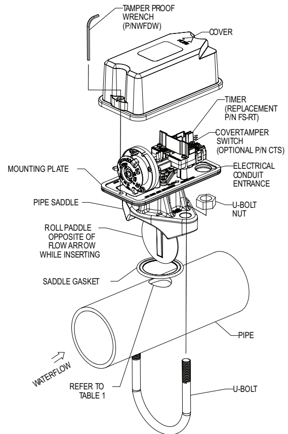
FIGURE 3. ASSEMBLY DIAGRAM:
