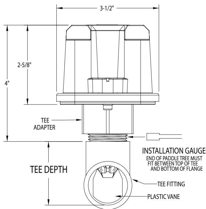
FIGURE 1. MOUNTING DIMENSIONS
