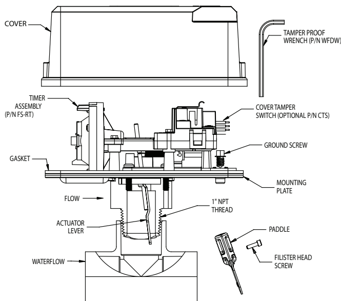
FIGURE 2. ASSEMBLY DIAGRAM
